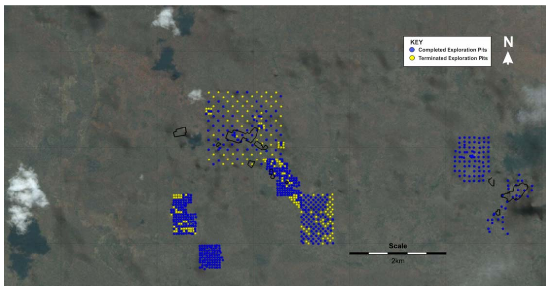
Figure 3-3: The completed (blue) and terminated (yellow) exploration pit collar locations shown relative to the current pit outlines (in black)
