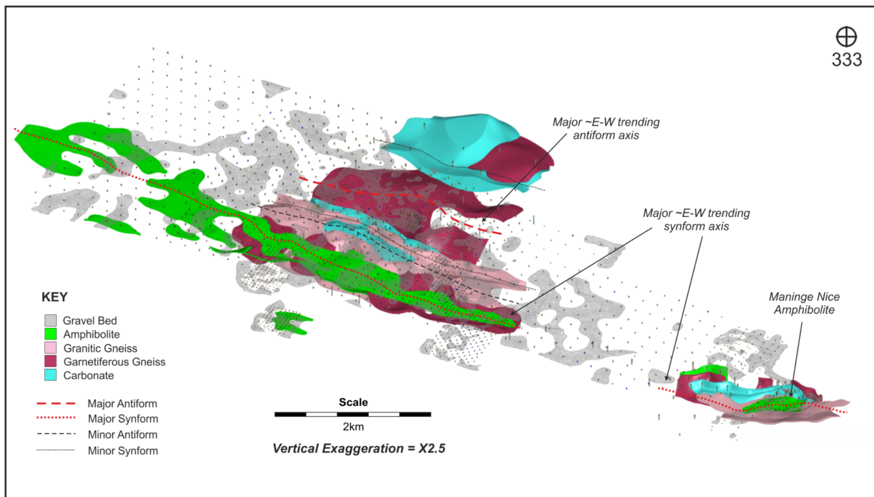
Figure 4-4: The Montepuez fresh rock model, overlain by the gravel bed resource model (in grey)
