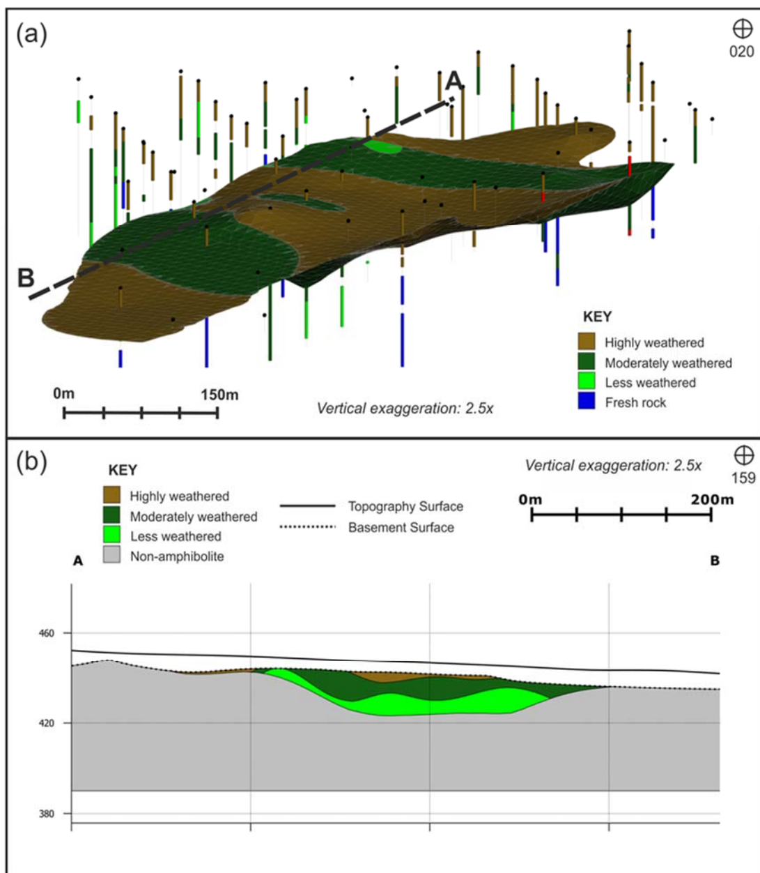
Figure 4-3: Oblique (a) and sectional (b) views of the Maninge Nice amphibolite model coloured by degree of weathering
