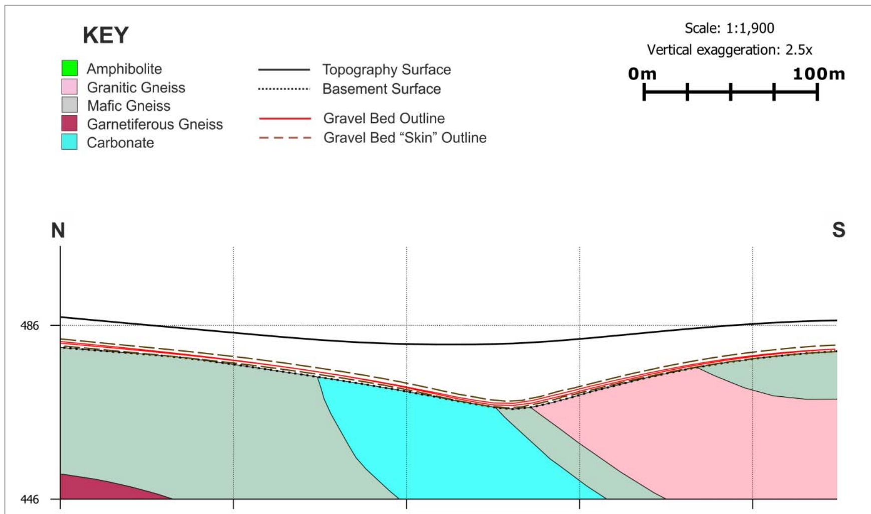
Figure 4-2: The modelled gravel bed (red) and gravel bed “skin” (dashed brown) shown relative to the basement geology model. Note that the gravel bed model broadly mirrors the trend of the basement surface
