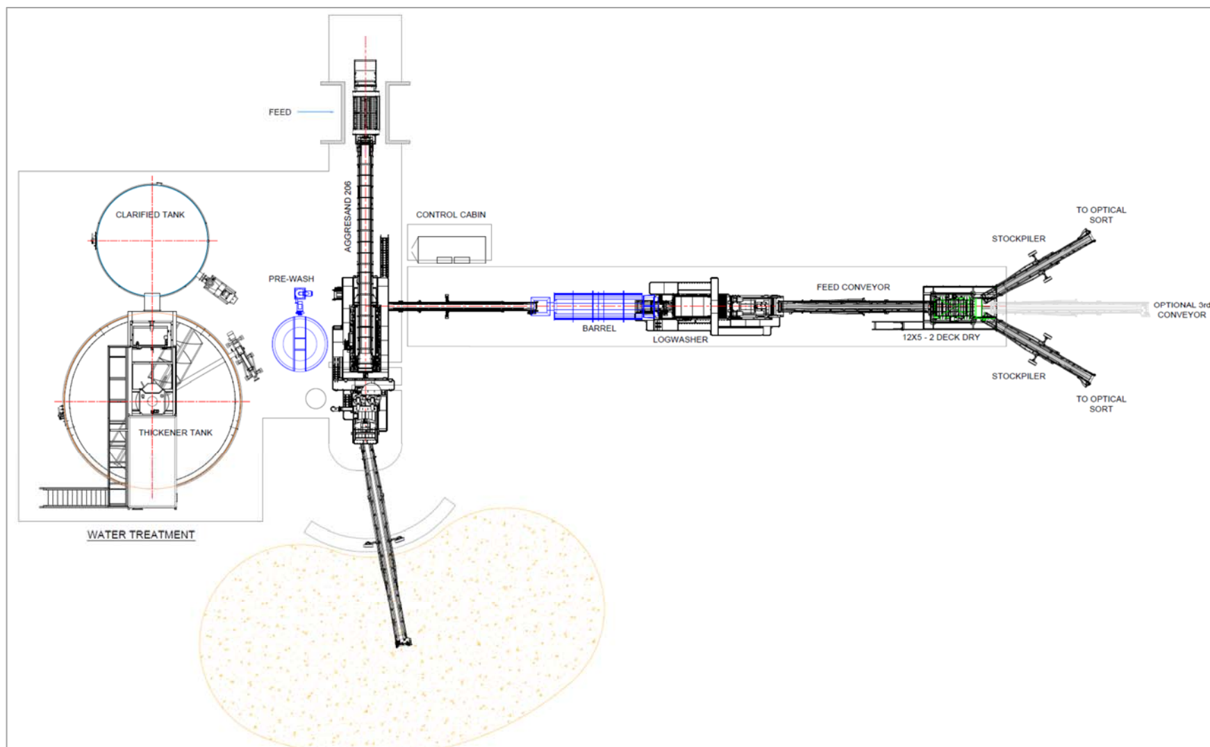
Figure 7-8: Conceptual layout for 250 tph plant
