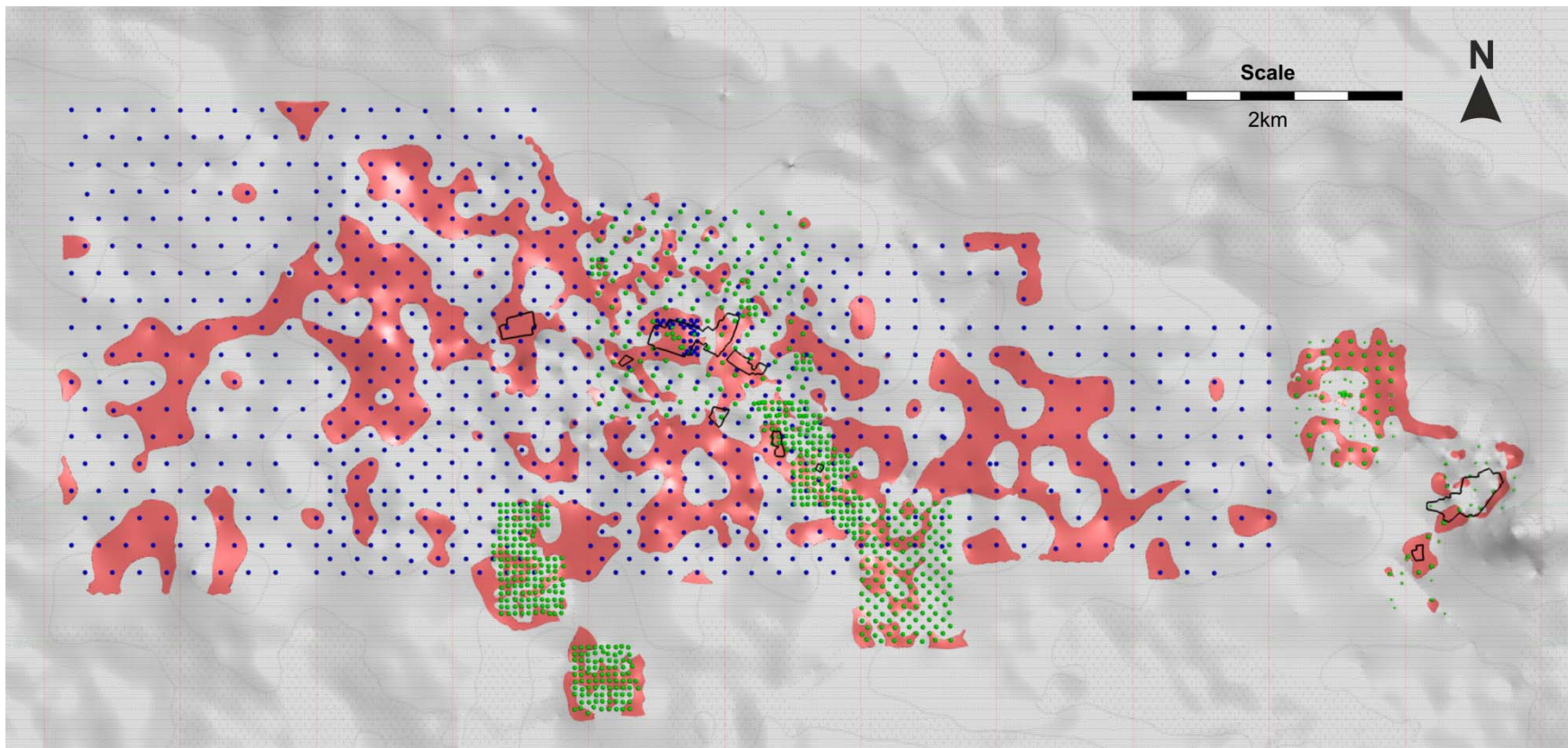
Figure 4-1: Plan view of the gravel bed model (in red) overlain on the basement surface, shown relative to the collar locations of auger drill holes (blue) and exploration pits (green)
