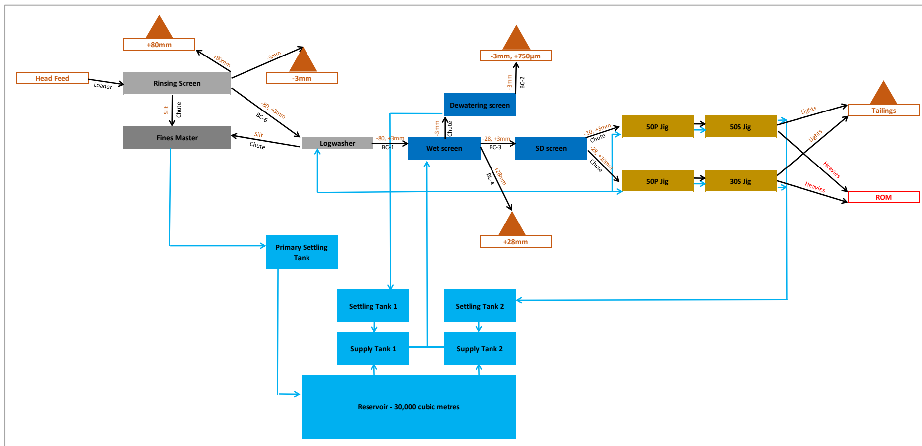
Figure 7-1: Existing plant flow sheet
