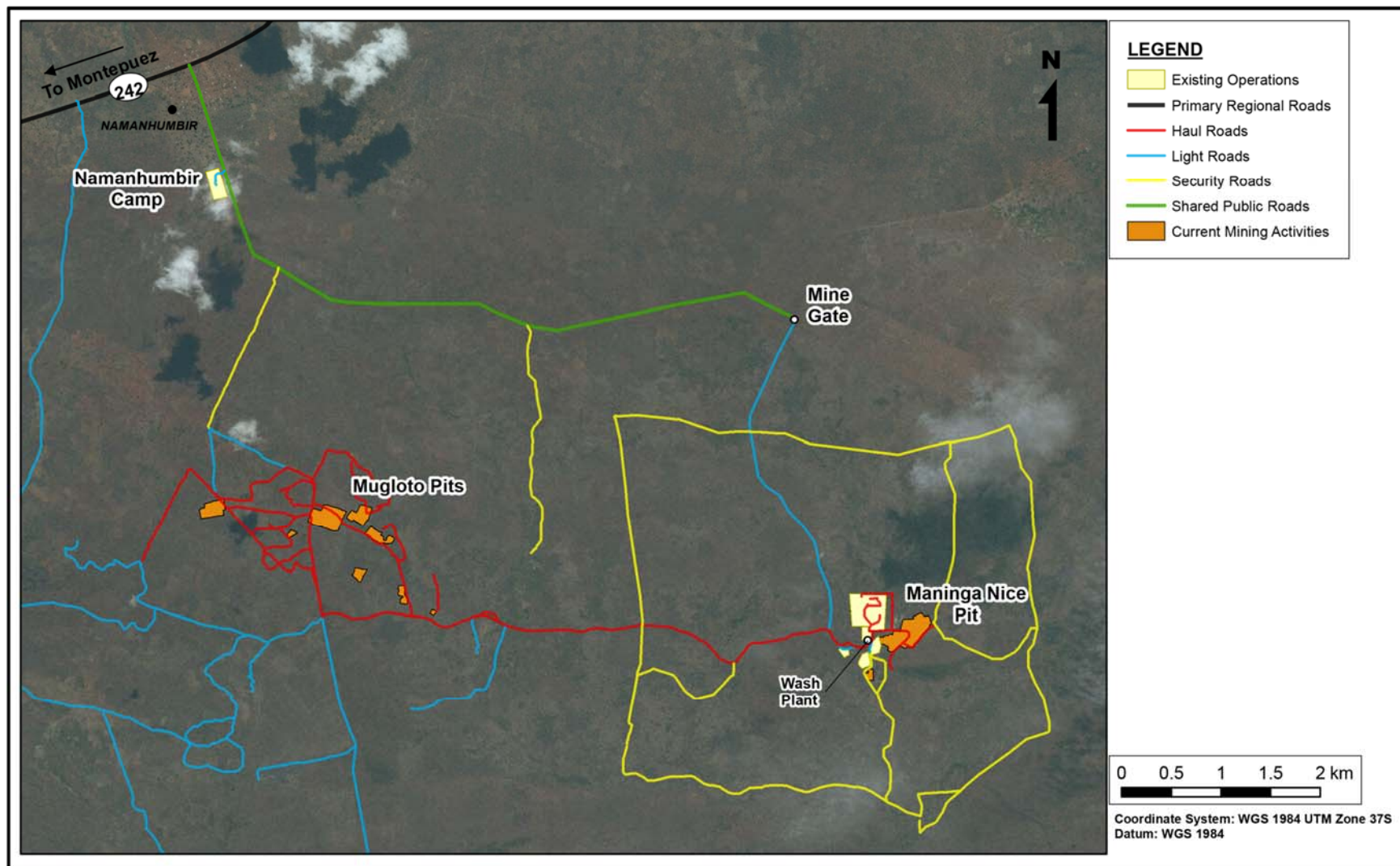
Figure 8-1: Existing Project Layout
