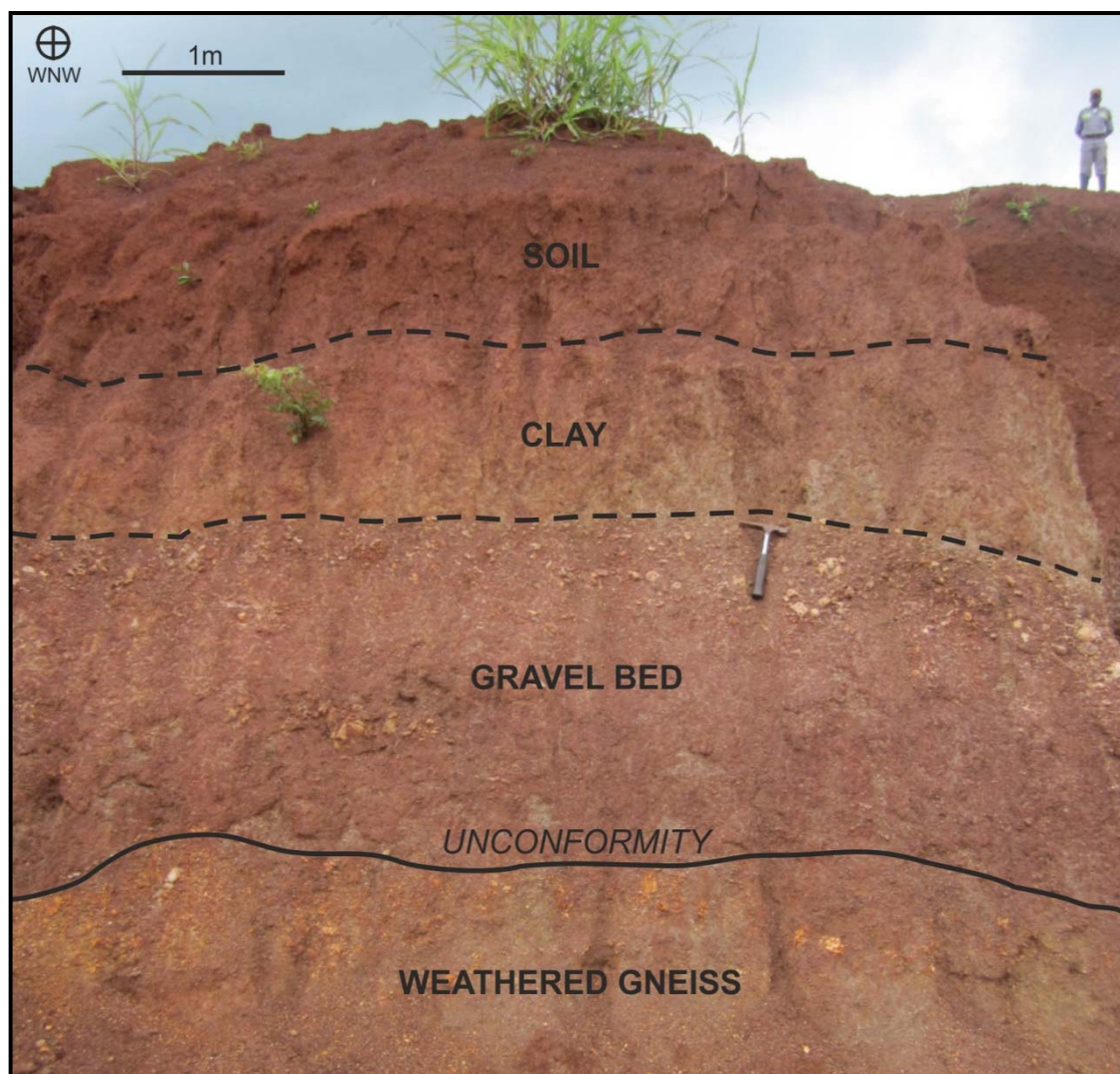
Figure 2-5: Overburden stratigraphy at the west face of Mugloto Pit 3
